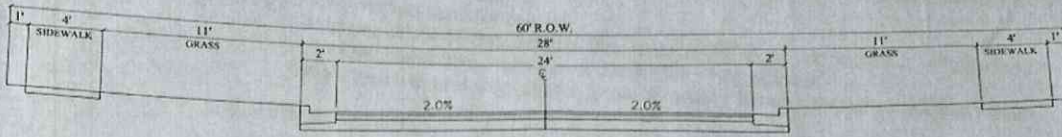
Collector Street with curbs and gutters
