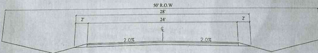
Local Street without curbs and gutters
